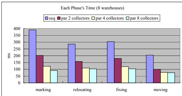
Figure 8: Scalability of parallel non-LOS compaction
