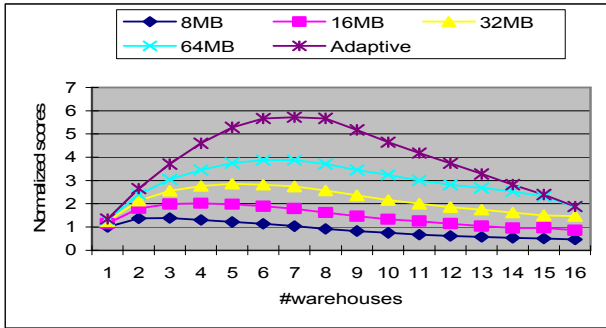
Figure 7: SPECjbb2005 performance with different NOS sizes
