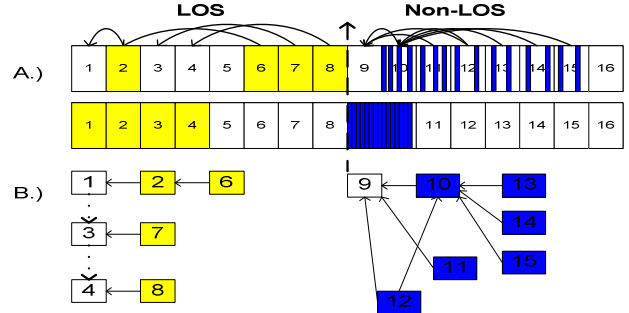
Figure 3: Partitioning of the heap into equal-sized blocks a.) By dividing the spaces into equal-sized blocks. Both false data dependencies and synchronization costs can be reduced. b.) to capture all data dependencies and to facilitate the parallelization of data compaction, dependency lists are generated for LOS and a dependency tree is generated for non-LOS. Note that in non-LOS, one target block can have multiple source blocks and one source block can have up to two target blocks. In LOS, one target block has only one source block, and vice versa. Note the block sizes for LOS and non-LOS can be different, but they are equal within either space.
