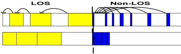
Figure 2: normal and large object compaction There are strong data dependencies in LOS such that the second object cannot be moved until the first object has been moved out, and the third object cannot be moved until the second one has been moved out, in this case, no parallelism can be exploited. In non-LOS, object movement can be highly parallel since the object size is smaller hence less interdependence between individual object. And in most cases, there is more free space than live objects. However, fine-grain parallel data movement in non-LOS imposes high synchronization overhead.
